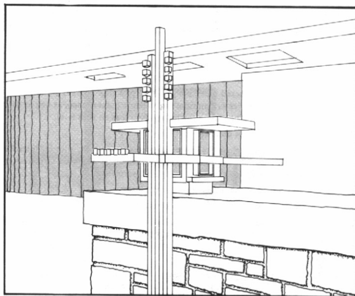
Lamp Detail
