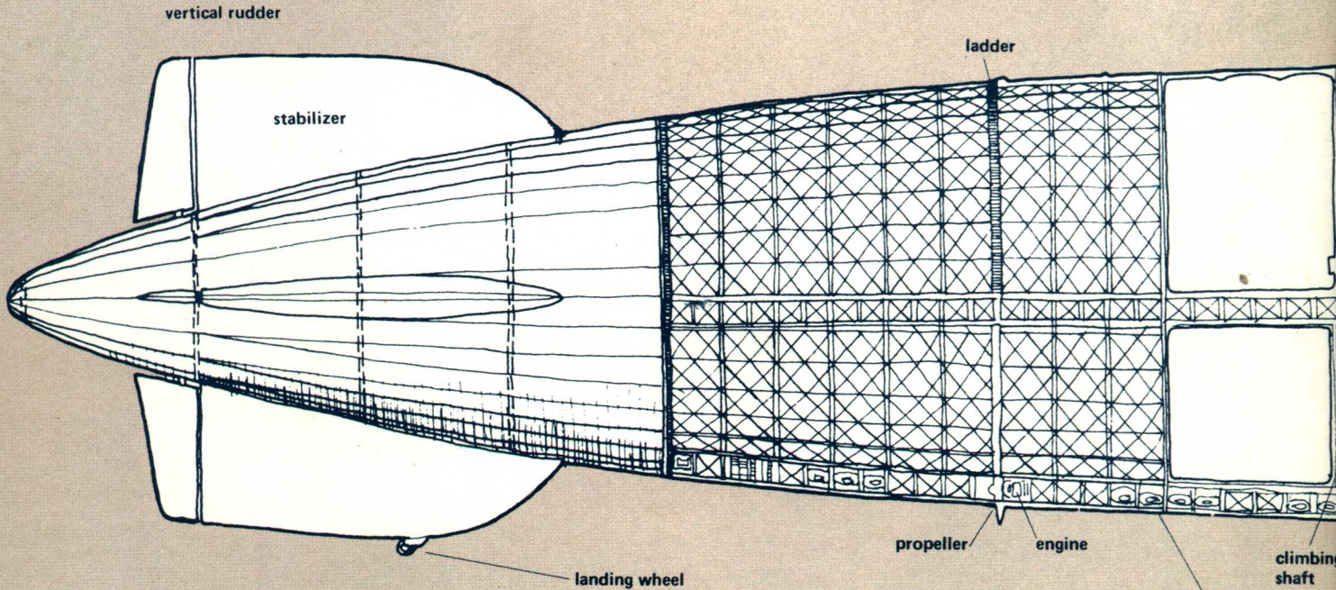
Side View, HINDENBURG
