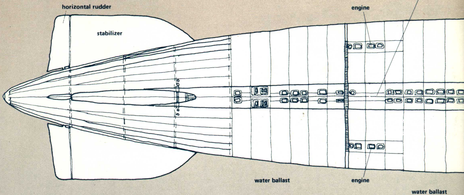
Bottom View, HINDENBURG
